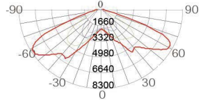
AVERAGE BEAM ANGLE(50%): ASYMMETRIC 80*140 DEG
