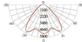
AVERAGE BEAM ANGLE(50%):90 DEG
