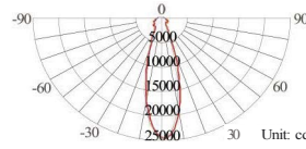
AVERAGE BEAM ANGLE(50%):30 DEG
